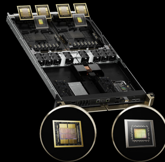
GB200 Superchip Compute Node
