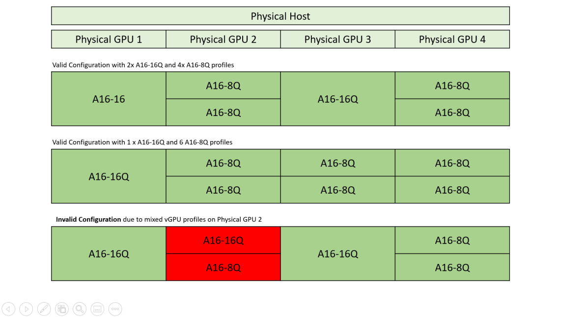
Figure 2.2 Example vGPU Configurations for NVIDIA A16
