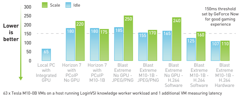
Figure 3. Click to Photon Latency at scale under various scenarios with and without a GPU
