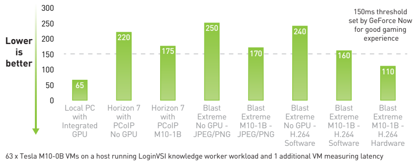
Figure 2. Click to Photon Latency under various scenarios with and without a GPU
